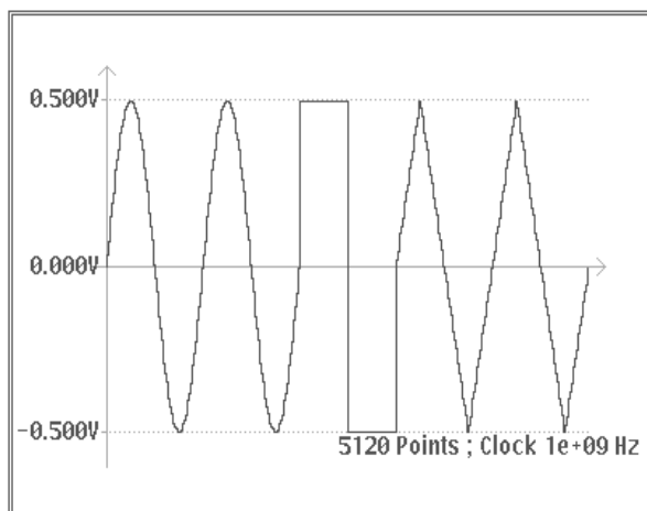
Figure 4A-122: Sequence File Data and Sample Waveform Display
