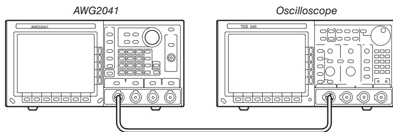
Figure E-8: Burst Mode Initial Test Hookup
