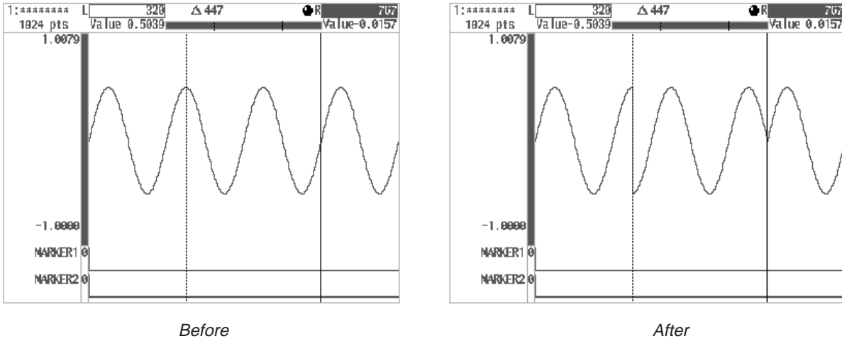
Figure 4A-36: Vertically Inverted Display
