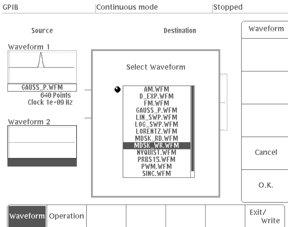
Figure 4A-148: Selecting a Waveform File
