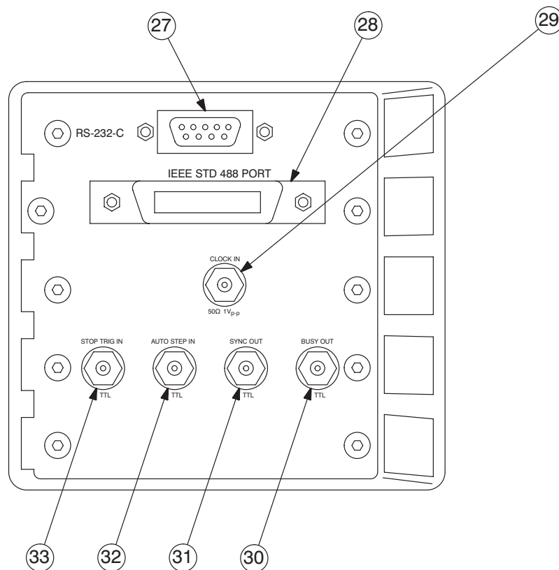
Figure 2-5: Rear Panel Detail
