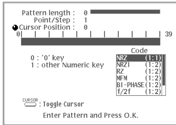
Figure 4A-39: Entering Pattern Data
