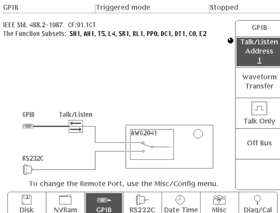
Figure 4E-9: Menu Displayed When GPIB is Selected
