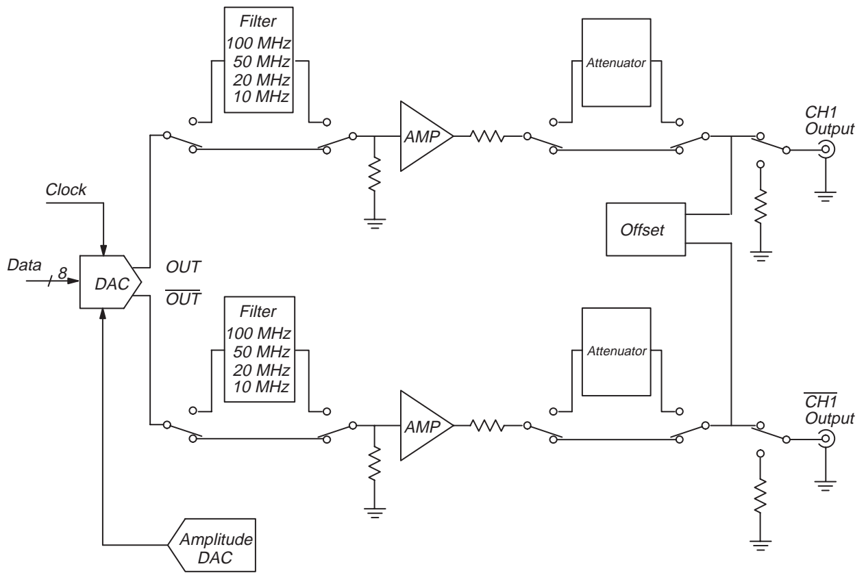
Figure 3-2: Block Diagram (2)
