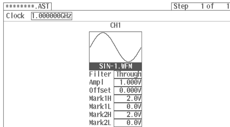
Figure 4A-134: Setting a File
