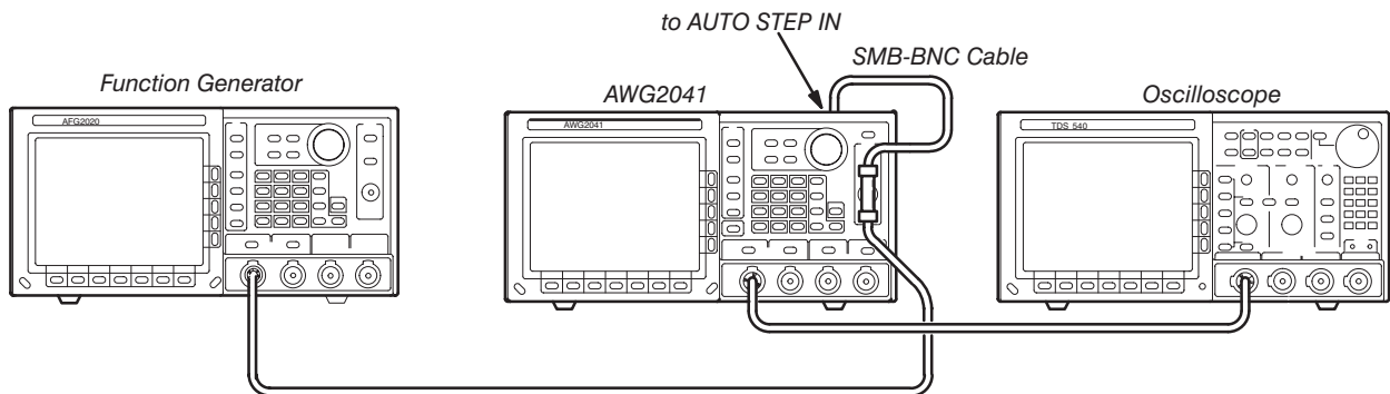
Figure E-11: Autostep Mode Initial Test Hookup
