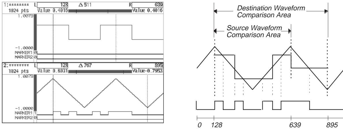
Figure 4A-73: Comparison Without Hysteresis
