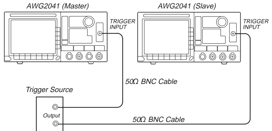
Figure 3-5: Sample Connection 2
